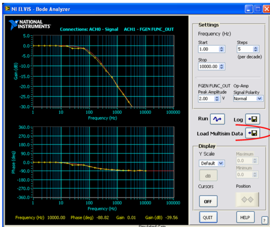
Figure 5.4: NI ELVIS Bode Analysis Comparing MultiSim Data
