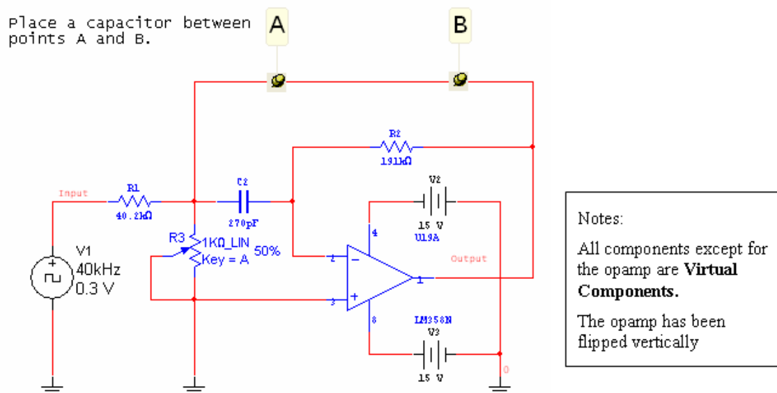
Figure 2.17: Bandpass Filter
