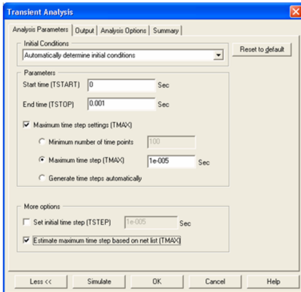
Figure 4.34: Setting Up the Transient Analysis
