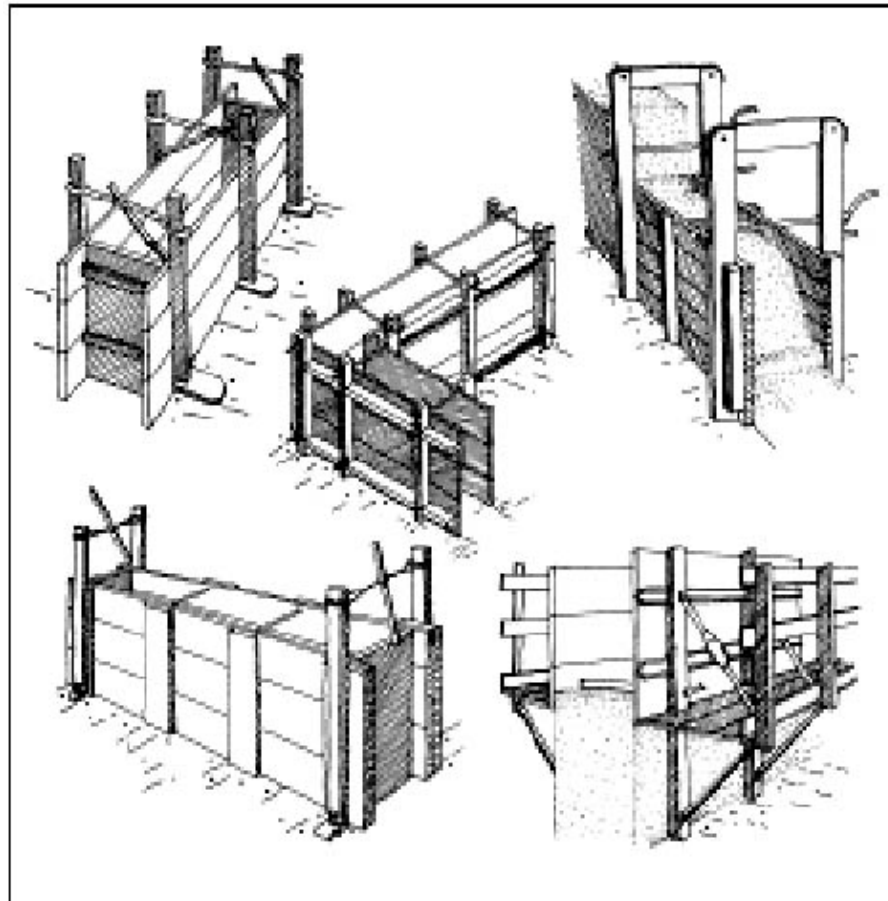
6-3 Formwork for rammed earth (Minke 2000)
