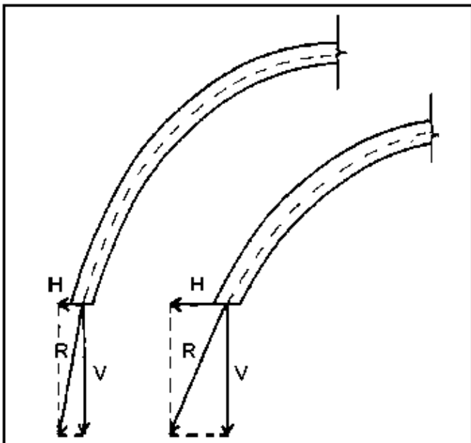
14–1 Resultant forces and their components (Minke 2000)
