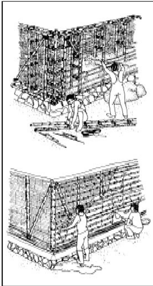
8-2 Wattle and daub systems (after Vorhauer 1979)
