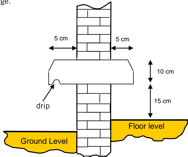
Figure 5: Termite barrier
