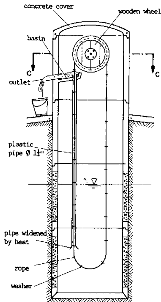
CROSS-SECTION A-A
