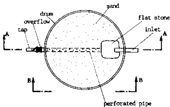
LAYOUT PLAN C-C
