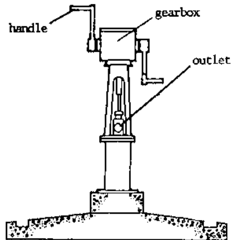
CUT-AWAY SIDE-VIEW
