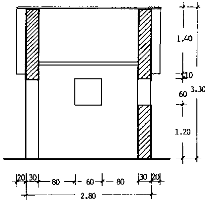
CROSS-SECTION B-B
