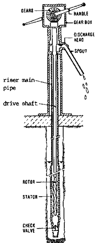
DETAIL OF PUMPING ELEMENT
