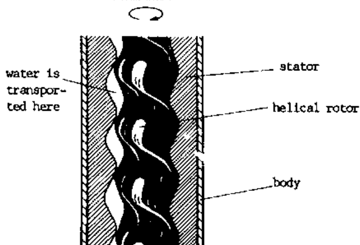
DETAIL OF PUMPING ELEMENT
