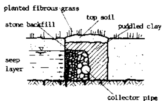
CROSS-SECTION A-A: INFILTRATION TRENCH
