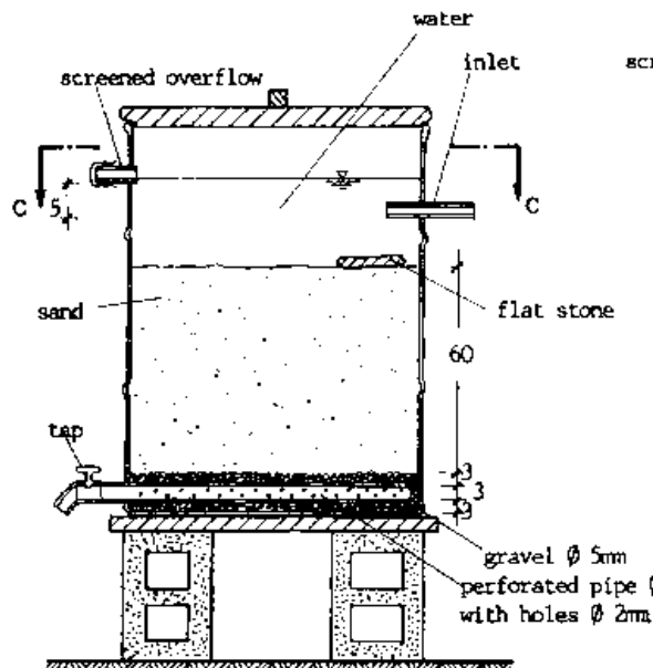
CROSS-SECTION A-A
