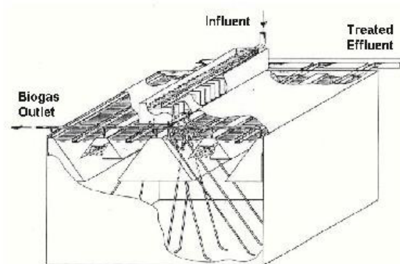
Fig. 4: UASB-reactor for domestic wastewater treatment, Mirzapur, India (Source: [4])
