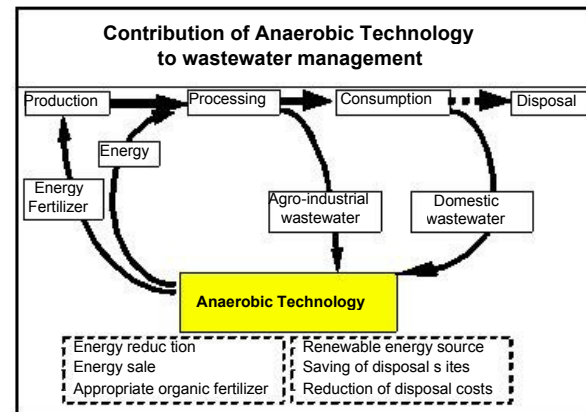
Fig. 3: Anaerobic technology for wastewater management
