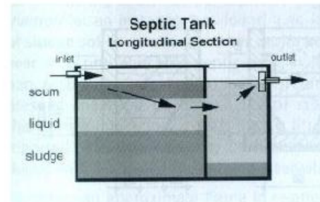
Fig. 6: Principle design features of septic tank (Source: [9])
