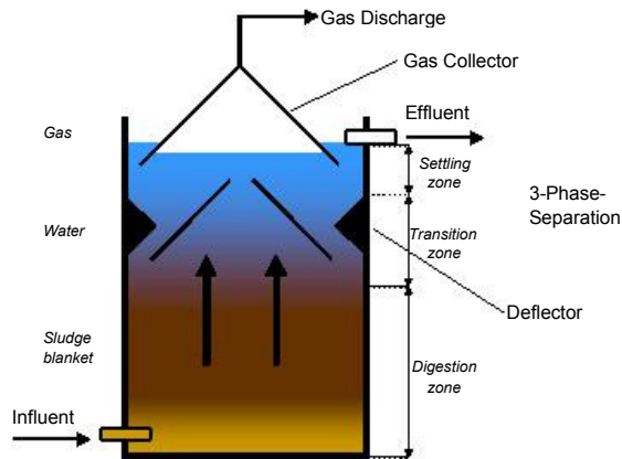
Fig. 5: Principle design features of UASB
