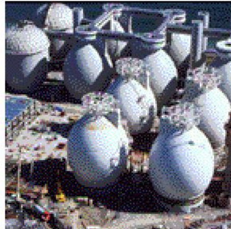
Fig. 7: Egg-shaped reactors for anaerobic sludge digestion (Source: TBW)
